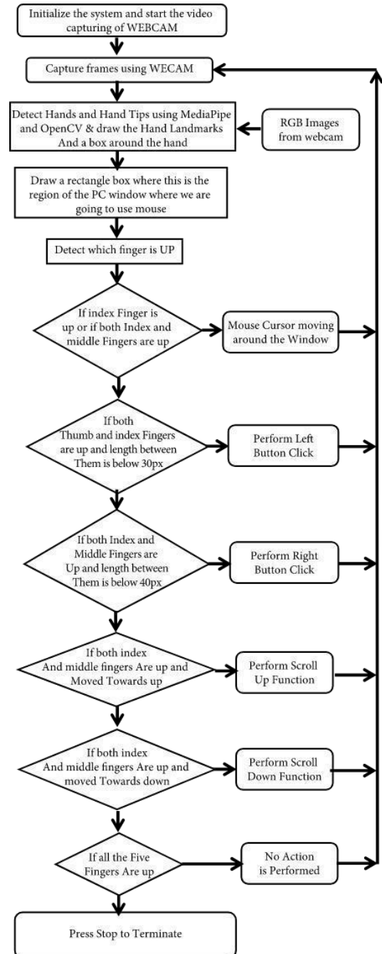
Fig. 2 Flowchart depicting the steps of performing gesture recognition
